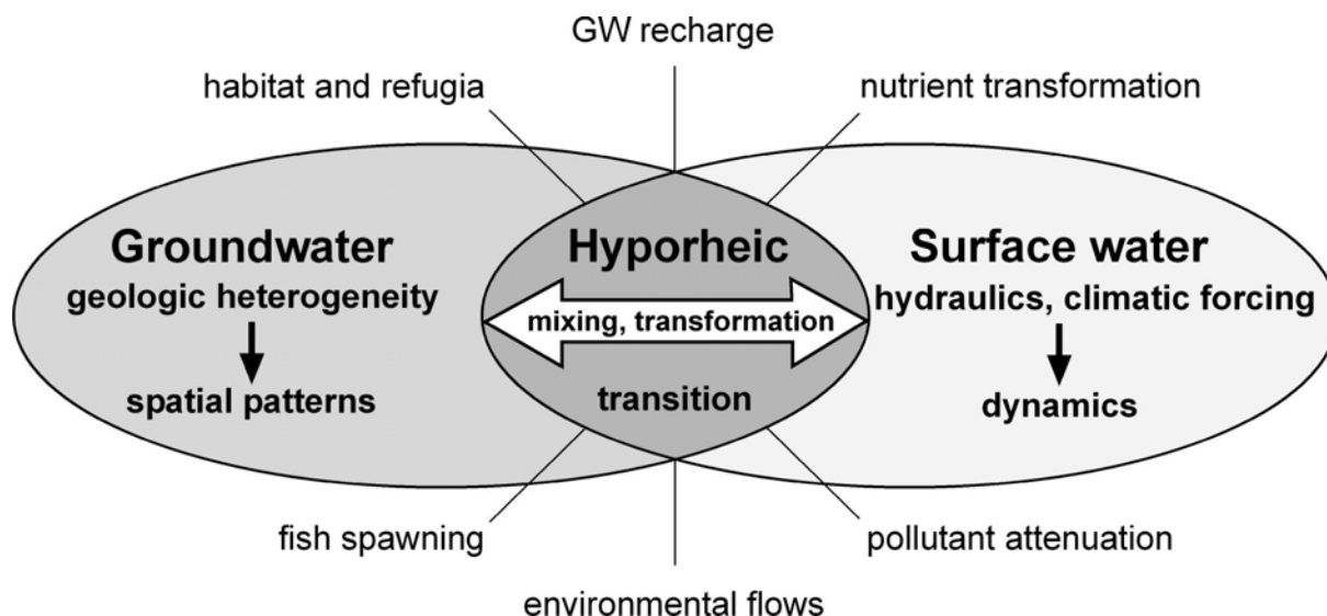
Figure 5.1 Hydroecological and biogeochemical functions of the hyporheic as a mixing and transition zone between groundwater and surface water environments, after Fleckenstein et al., 2008.
