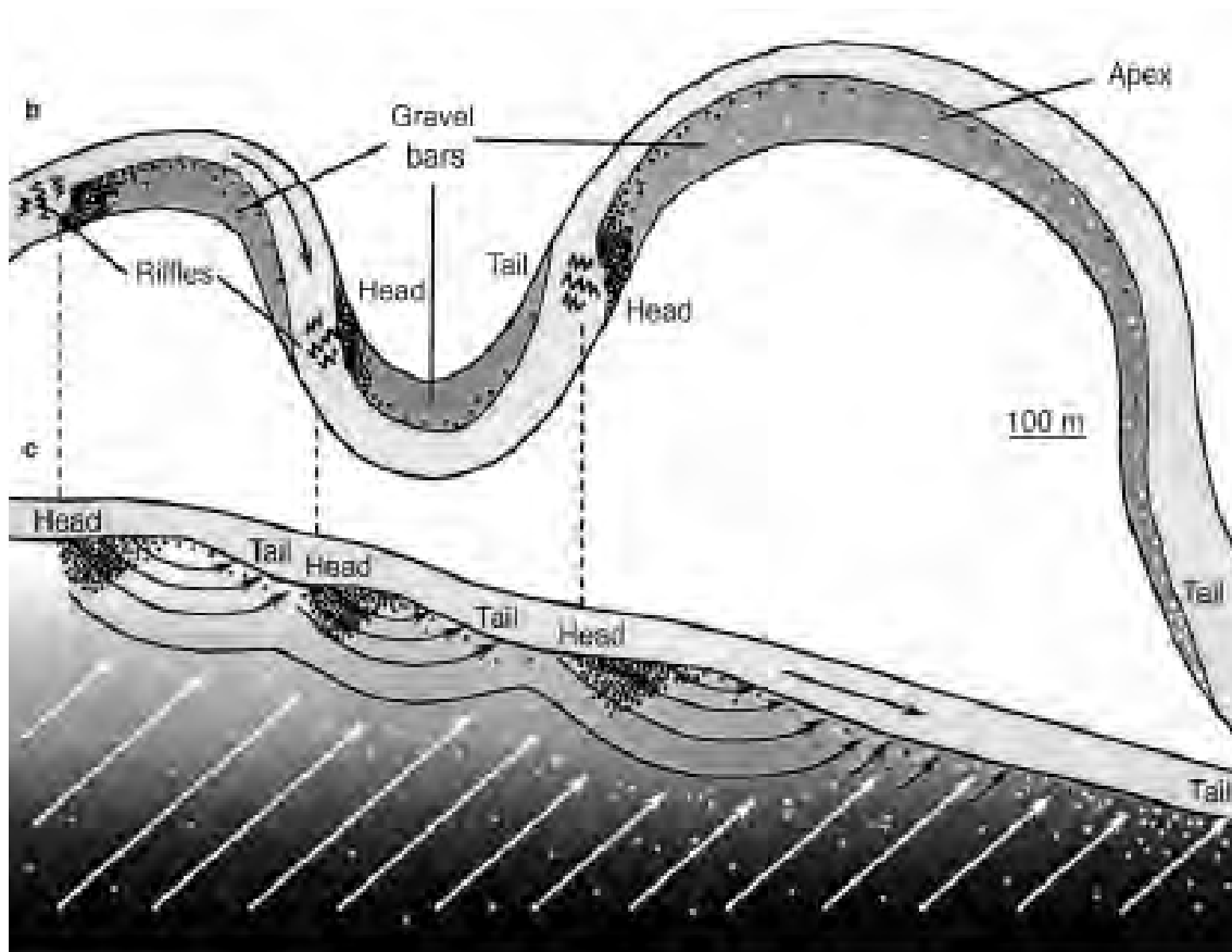
Figure 4.7 A conceptualization of river bed flows associated with riffled gravel bar reaches [Malcolm et al. (2003), after Malard et al. (2002)]. Only vertical flows are shown: in addition, there will often be lateral flows into the surrounding alluvium that pass around the riffle and emerge again into the channel downstream; there will also be flows that pass across the meander loop (see Figure 9). The deep groundwater discharges (white arrows) will either pass around the outside of the shallow flows or discharge between one gravel bar and the next [cf. Figure 14 (b)].
