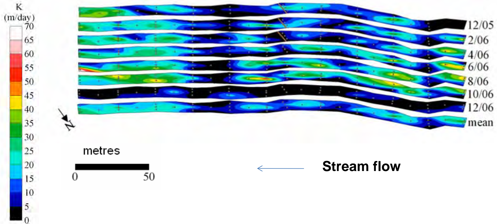
Figure 4.19 The variation in space and time of the permeability (K) of stream bed sediments as measured using a falling head method in a tube inserted 36 cm below the sediment surface along a reach of West Bear Creek, North Carolina, USA (Genereux et al., 2008). Measurements were taken between December 2005 and December 2006. The red line indicates a beaver dam, and the dots indicate measurement points.
