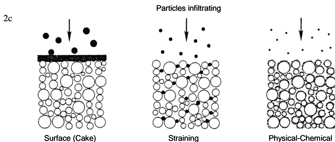
Figure 3.15 Sediment infiltration into river beds: a: Passive infiltration into a gravel bed; b: Relationship between gravel bed type and infiltrating sediment; c: Three filtration mechanisms for sediment infiltration into porous beds. Note the particle size dependence and difference in deposit morphology (Modified from McDowell-Boyer et al. 1986 and Sear et al. 2008).
