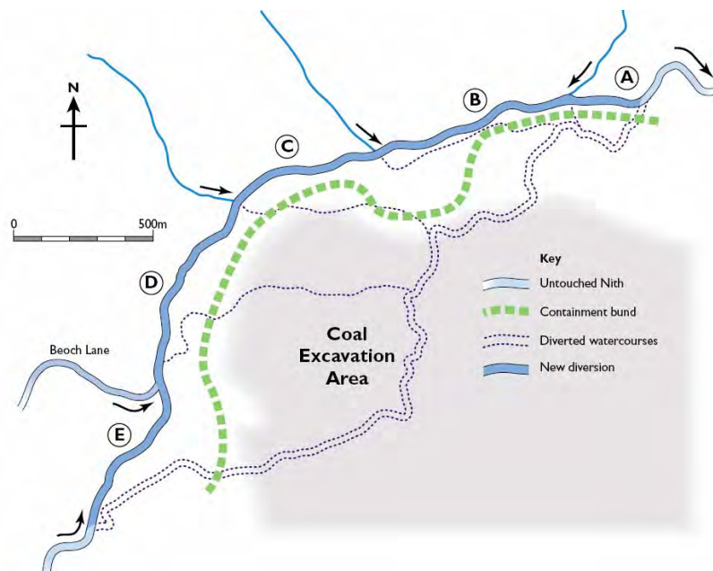
Figure 10.7 Diversion of a part of the River Nith away from expanding coal excavation (RRC 2007).
