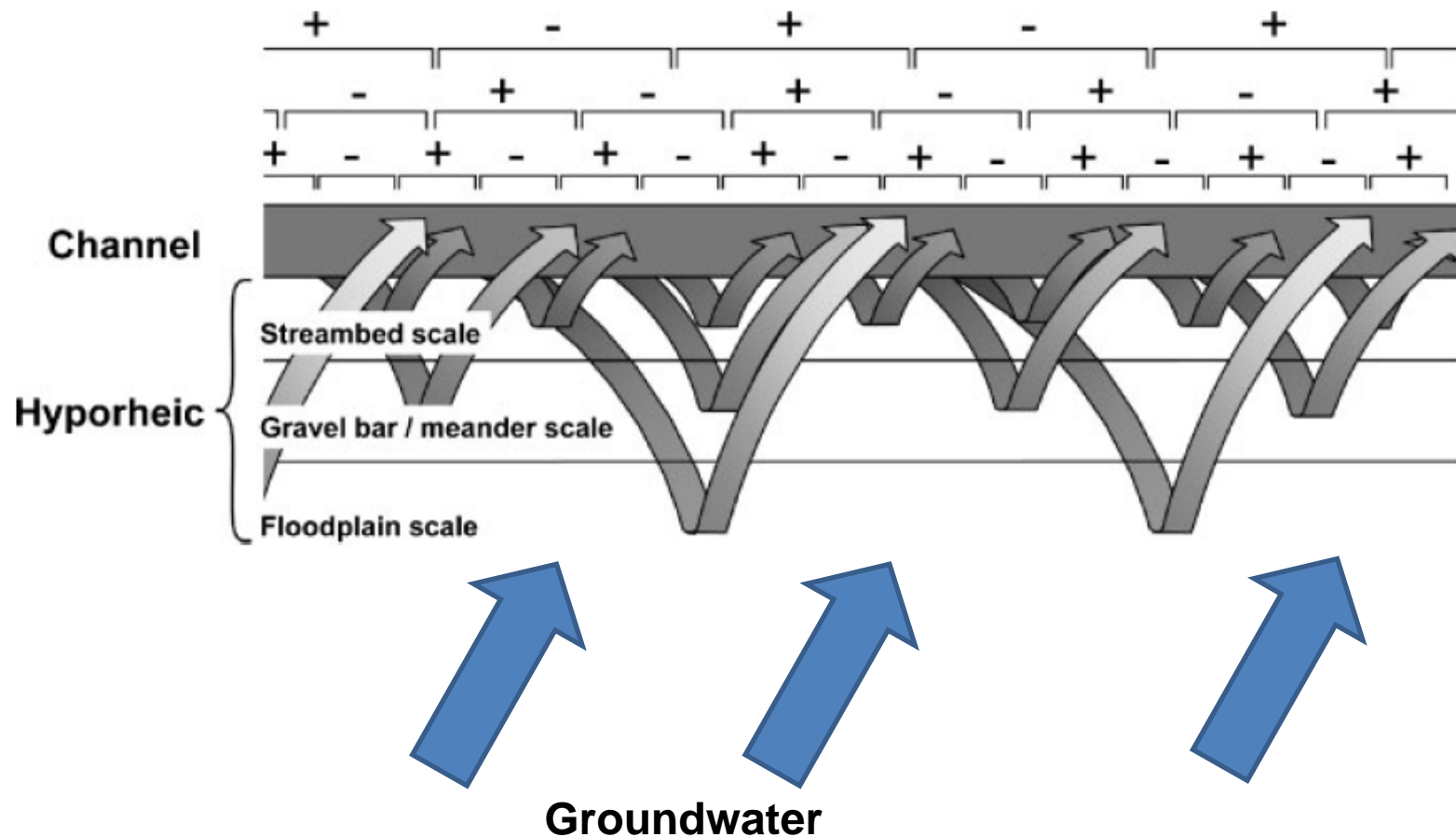
Figure 4.22 A cartoon illustrating the 'hydrologic spiraling' concept of Poole et al. (2008). The figure shows a longitudinal cross-section of a stream system with flows leaving and subsequently re-joining the stream on a variety of space (and time) scales. Changes in arrow shading indicate changes in water temperature and chemistry. Plus and minus signs indicate effluent and influent flow zones associated with each of the nested flow paths. In some cases there will be groundwater discharge (or recharge) also.
