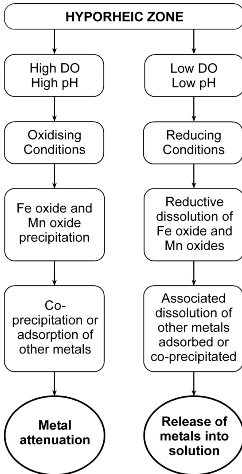
Figure 5.5 Generic redox and pH conditions for attenuation or release of mining-derived pollutants within the hyporheic zone (After Gandy et al., 2007).
