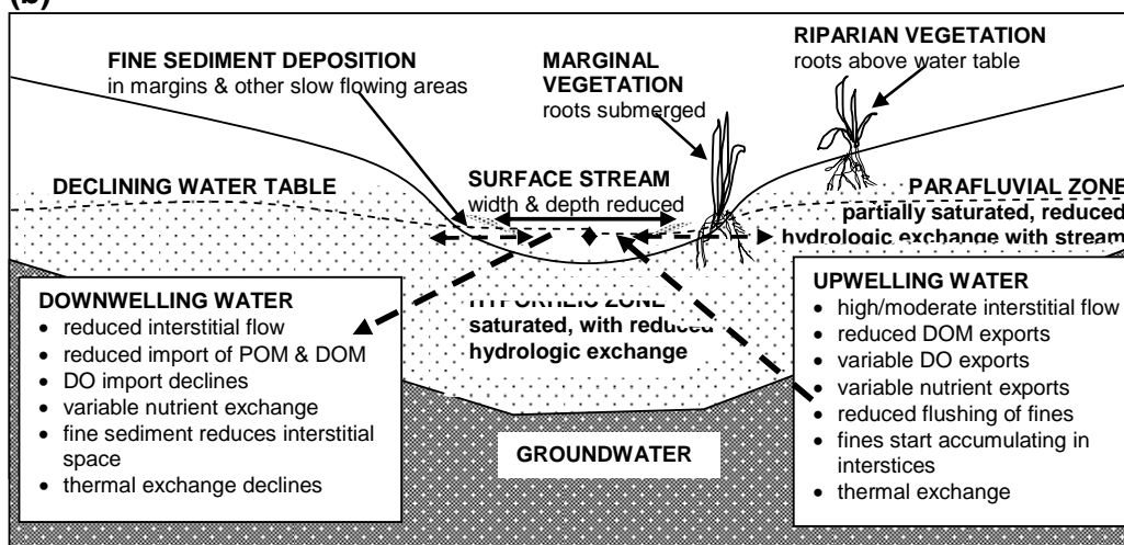
Figure 5.6 Conceptual model of ecologically significant processes and interactions between the benthic and hyporheic zones as a result of low flow and supra-seasonal drought (a) unimpaired flow and (b) low/base flow (After Stubbington et al. , 2009).
