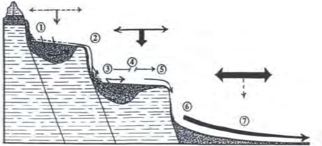
Figure 3.6 Zones of bedrock constriction and permeable alluvial deposits, showing deep penetration of surface water into the alluvium (Stanford and Ward, 1993).
